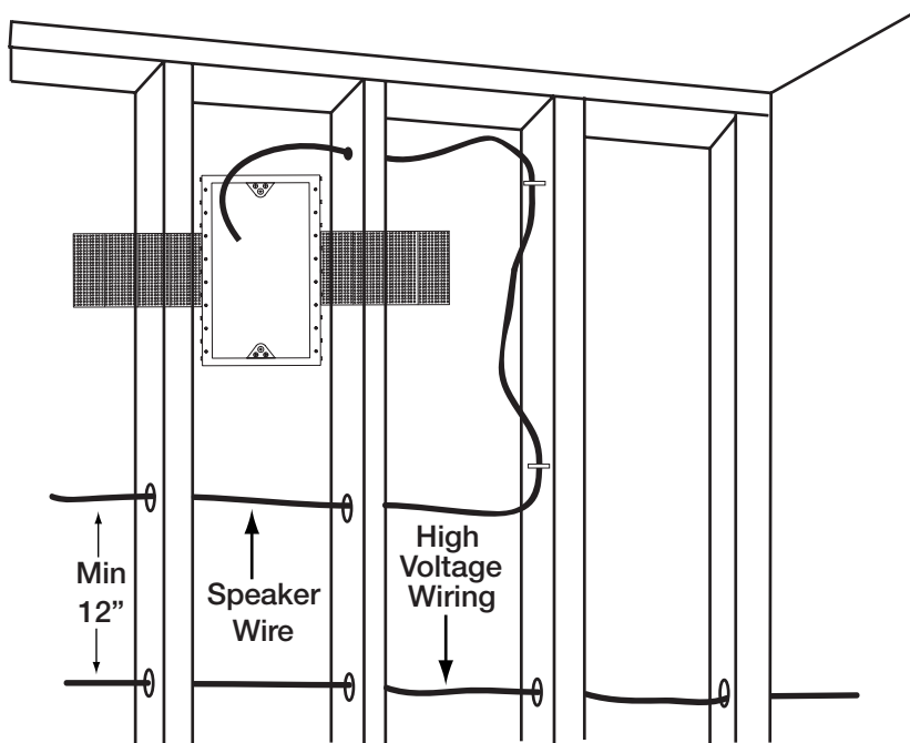
Figure 3.8 - Pre-Wiring
